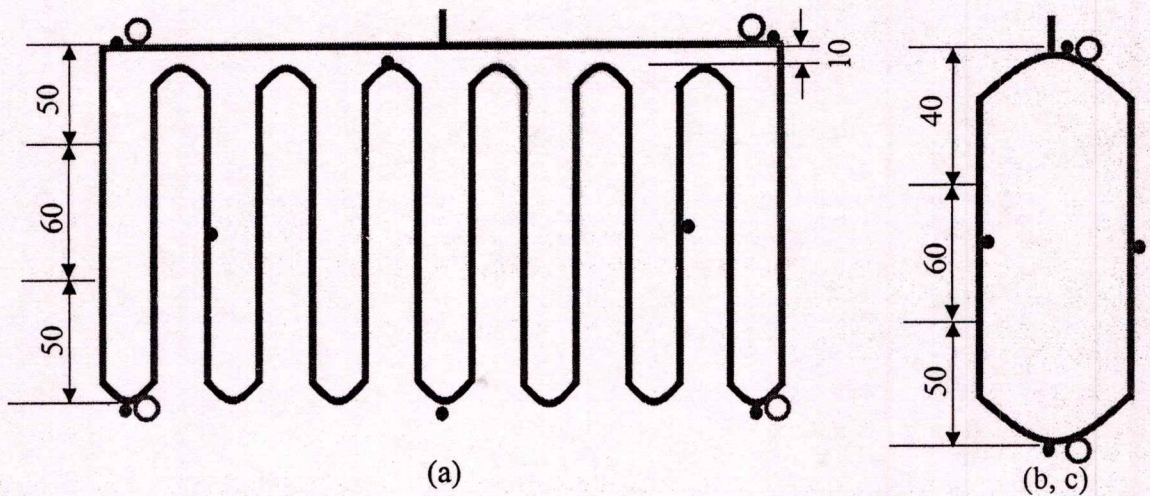
Figure 1: Schematic of the “Advanced Heat Pipe Demonstration Unit” experimental setup
