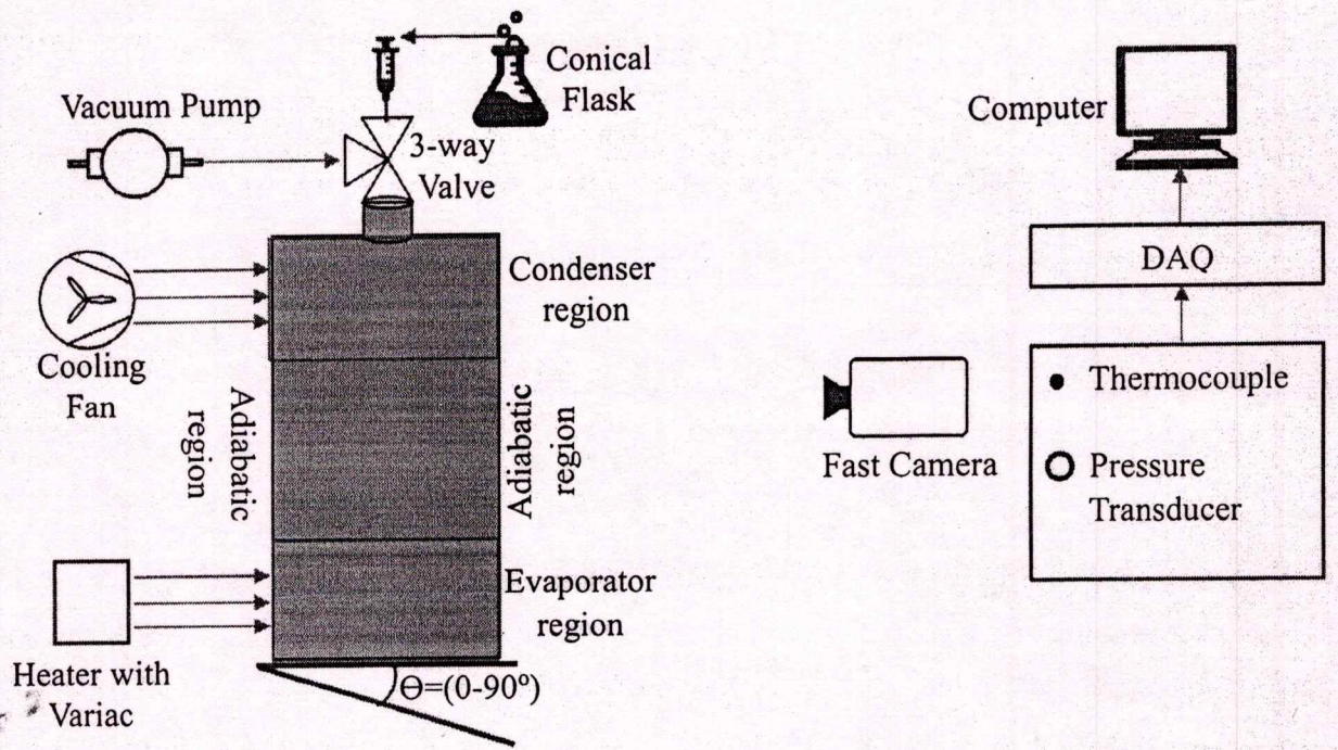
Figure 1: Schematic of the “Advanced Heat Pipe Demonstration Unit” experimental setup
